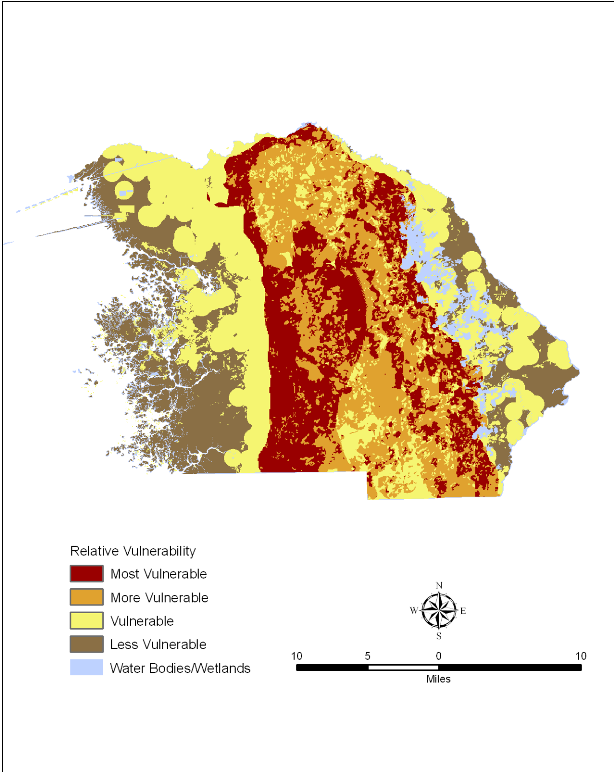
Figure 15. Relative vulnerability map for the Citrus County Aquifer Vulnerability Assessment project. Classes of vulnerability are based on calculated probabilities of a unit area containing a training point, or a monitor well with water quality sample results indicative of vulnerability.
