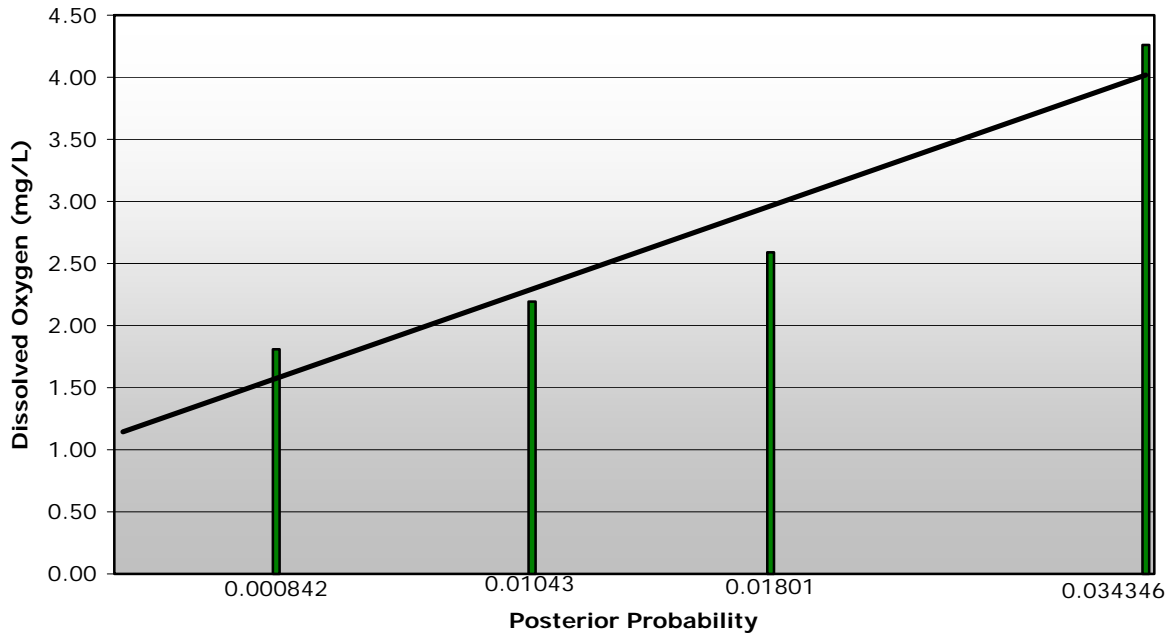
Figure 20. Dissolved oxygen values (averaged per posterior probability class) versus probability values to reveal trend between increasing dissolved oxygen concentrations and posterior probability.
