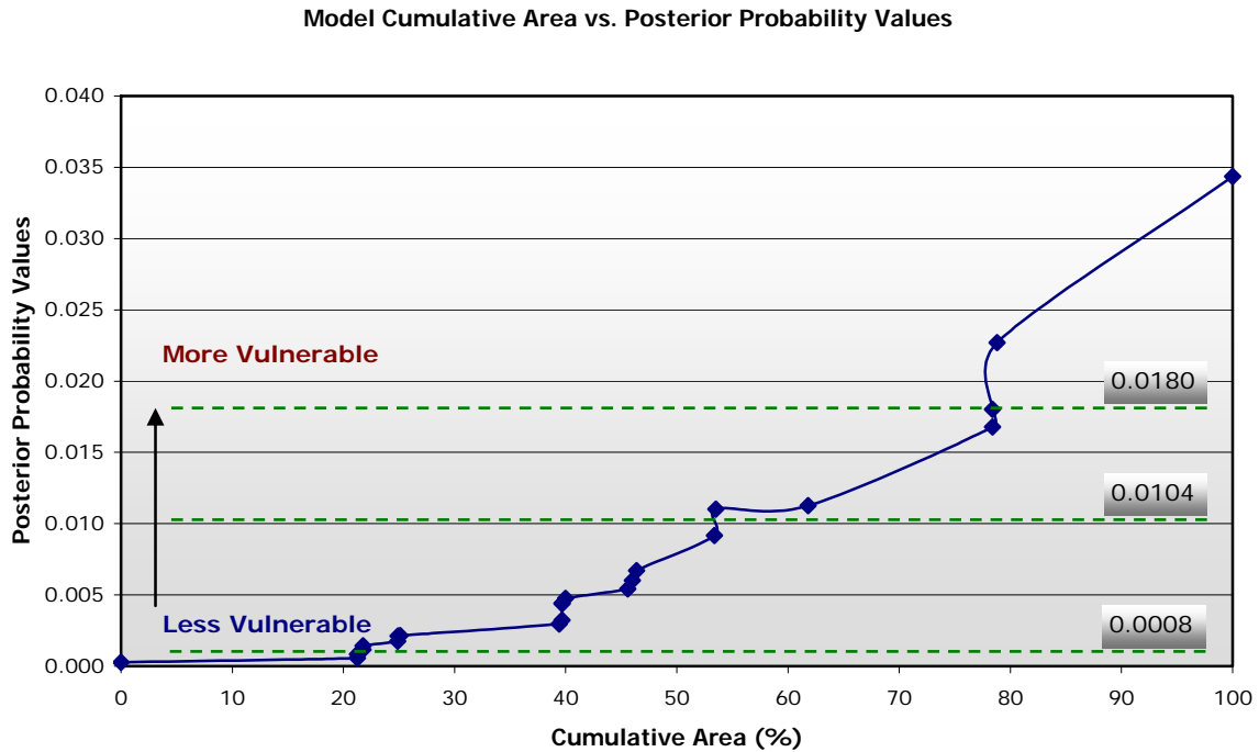
Figure 16. Vulnerability class breaks are defined by selecting where a significant increase in probability and area are observed.
